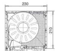
VEKAVARIANT 210 mm Revision unten
